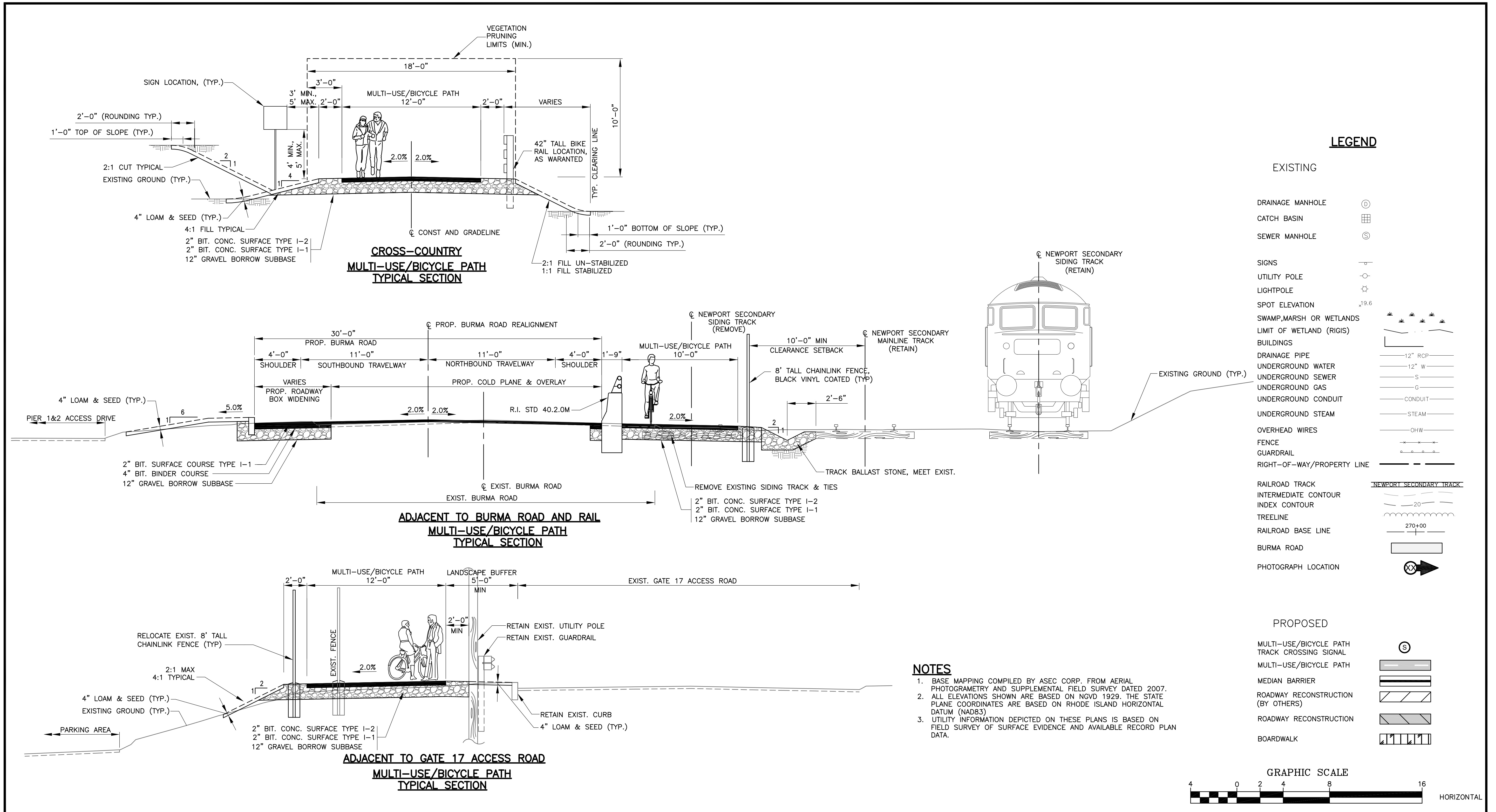
Figure No. 1 TYPICAL SECTIONS BURMA ROAD SEGMENT
